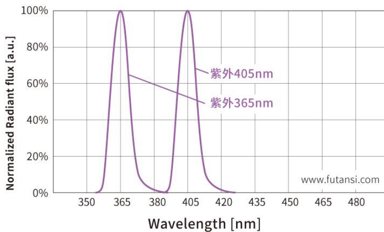
Fig 1. Spectrum, T_s=25^\circ\text{C} , I_f=1\text{A}
